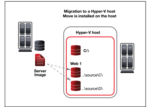
Hyper-V Configuration
