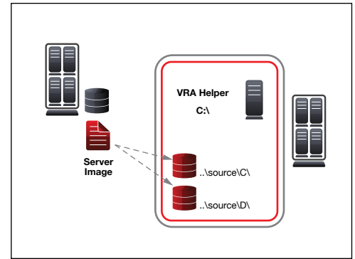
VMware Configuration
